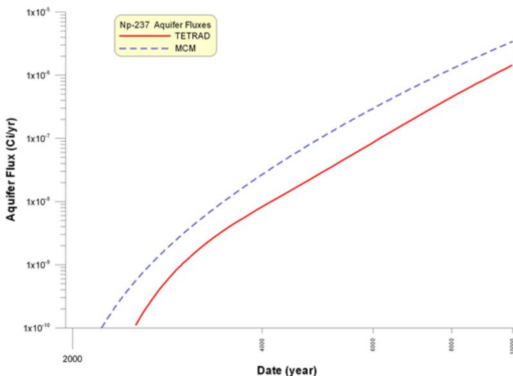
Figure 3-14. Example Results Comparing Fluxes Obtained from a 3D Model with Fluxes Predicted Using an Abstraction to an 1D Equivalent Model and Illustrating Pessimistic Bias of the Simplified Model
