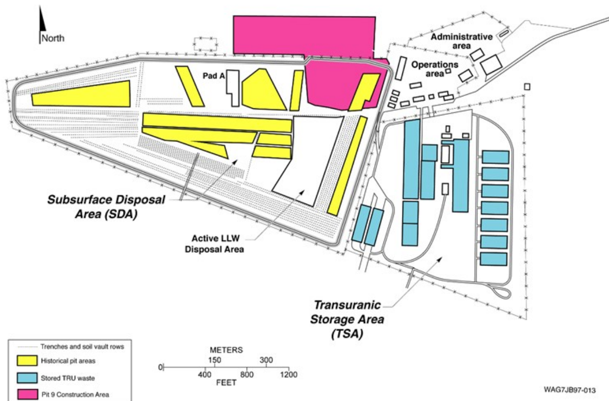
Figure 3-4. Example of Active Disposal Facility and Co-Located Historical Disposal Locations
