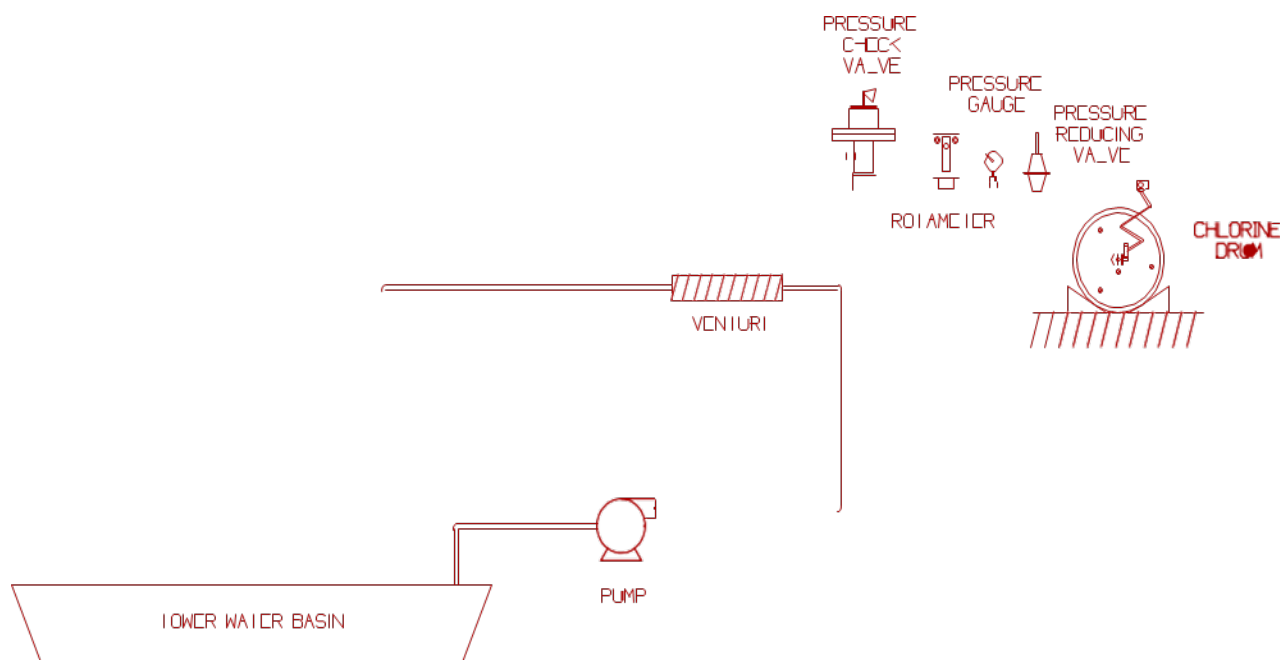
FIGURE 4.2. Cooling Water Chlorination System
